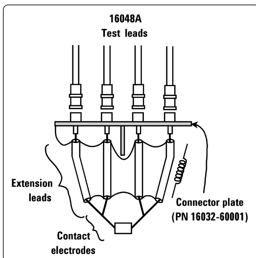
Figure 2 . Contact electrodes
