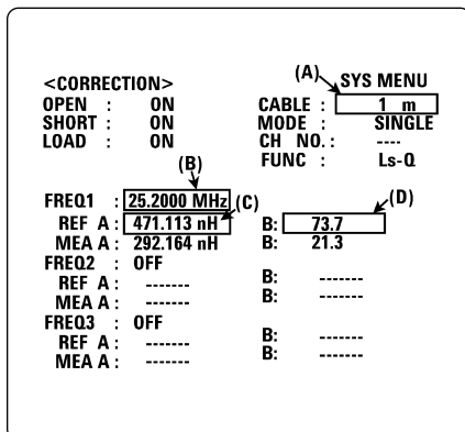
Figure 3. Correction function setup
