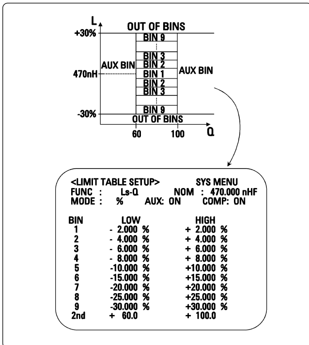
Figure 5 : Comparator setup
