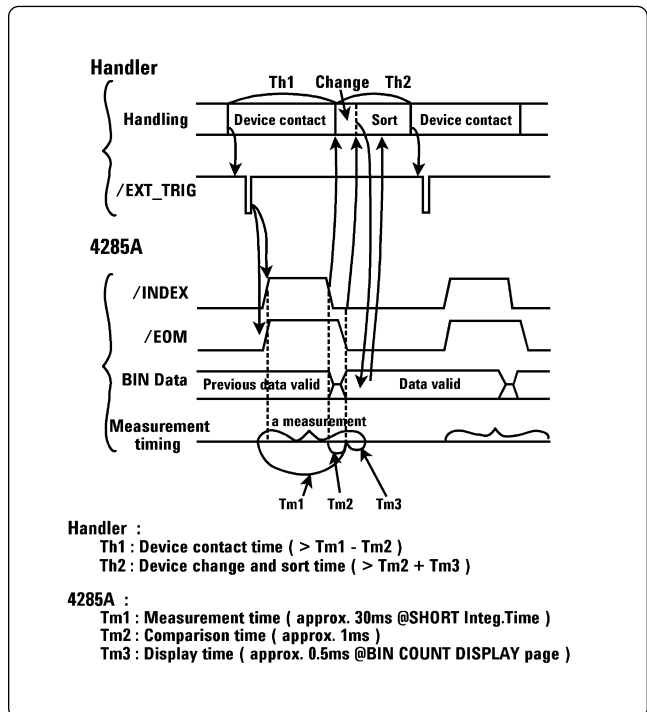
Figure 6 : Sample interface timing chart
