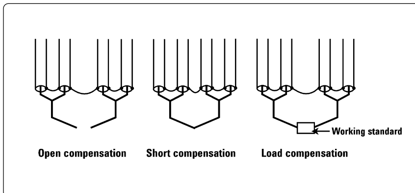
Figure 4. Performing correction measurements
